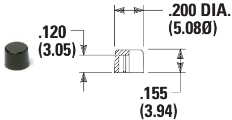
Cap, 0.120" DIA. Plungers
