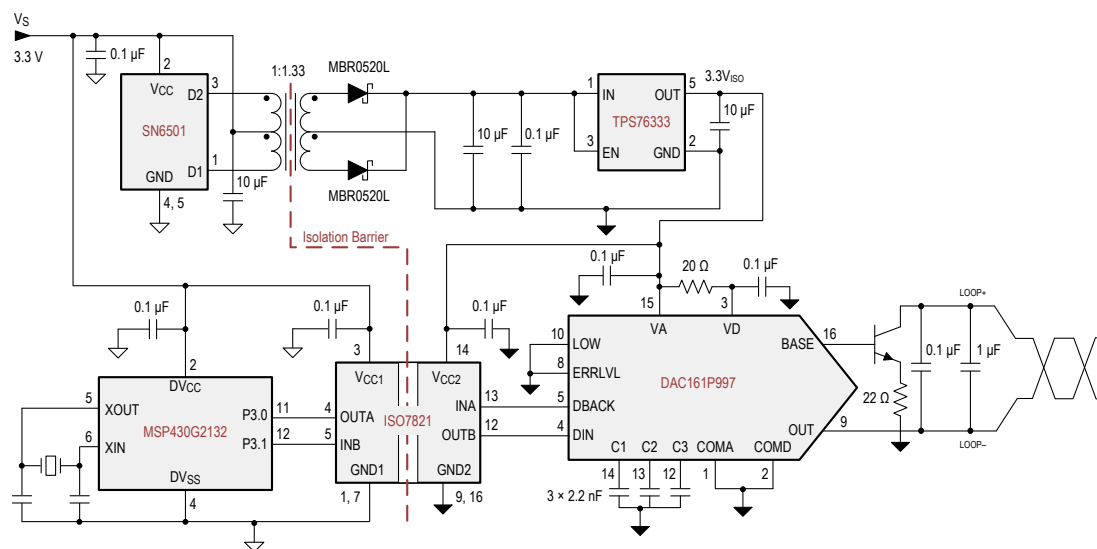
Figure 16. Isolated 4-20 mA Current Loop
