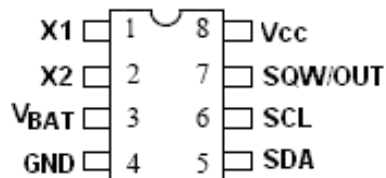
DIP-8/SOP-8/MSOP-8
