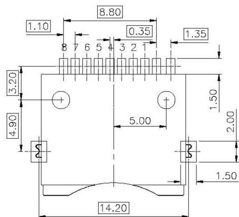
RECOMMENDED P.C.B LAYOUT(TOP VIEW) GENERAL TOLERANCE \pm 0.05
