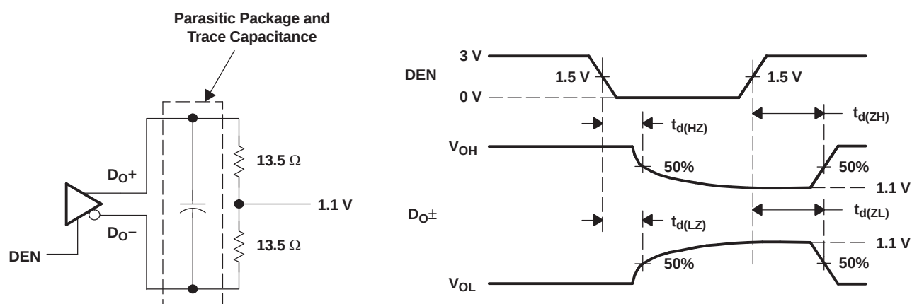
Figure 10. Serializer High-Impedance State Test Circuit and Timing
