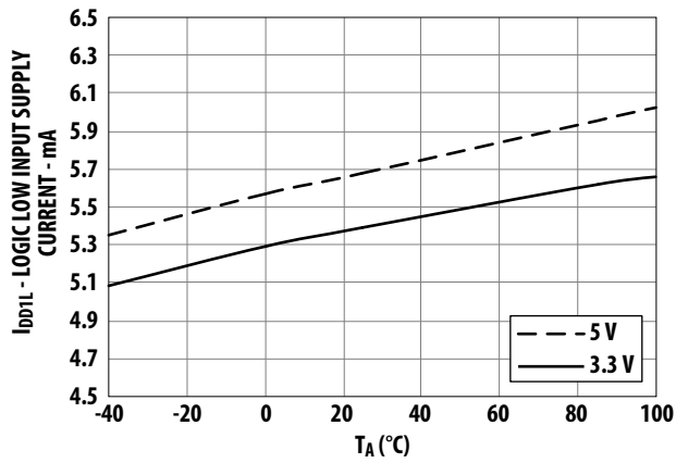
Figure 1. Typical Logic Low Input Supply Current versus temperature.
