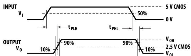
Figure 12. Signal plot shows how propagation delay is defined
