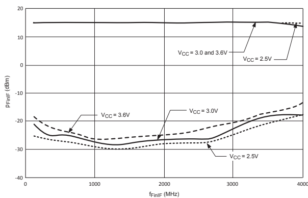
Figure 4. IF PLL Fin Sensitivity
