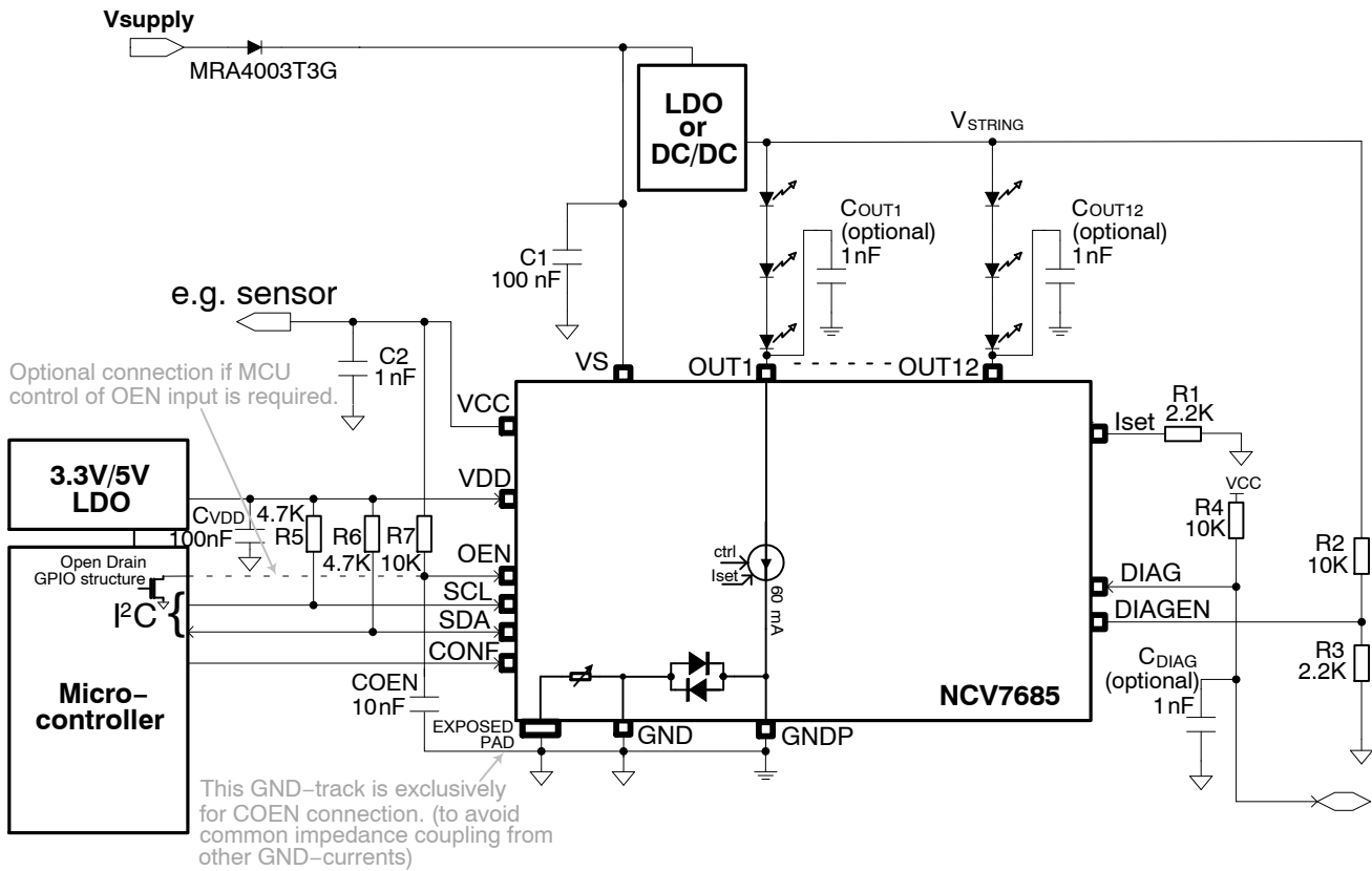
Figure 4. Application Diagram with Micro-controller (I²C Mode)
