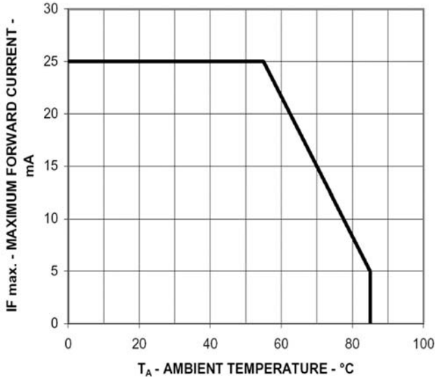
Figure 6: Derating Curve
