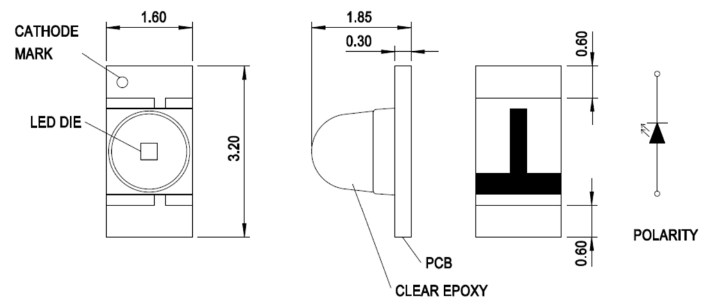
Figure 1: Package Dimensions
