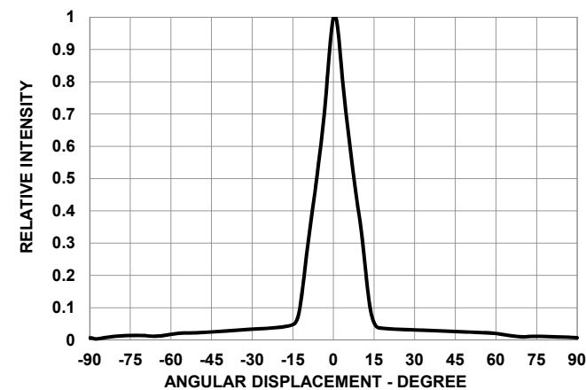
Figure 5: Radiation Pattern
