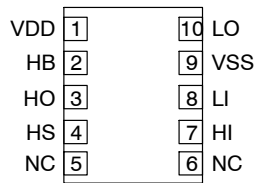
WDFN10
