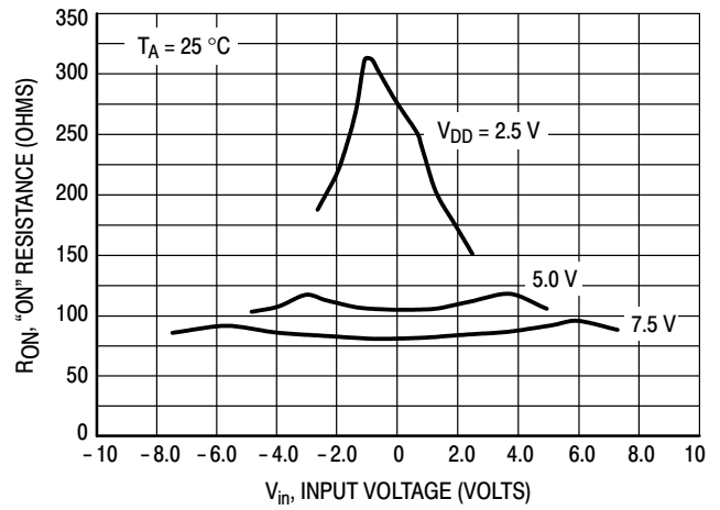
Figure 13. Comparison at 25\text{ }^{\circ}\text{C} , V_{DD} @ - V_{EE}
