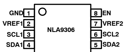
Figure 2. US8/TSSOP-8 Pinouts
