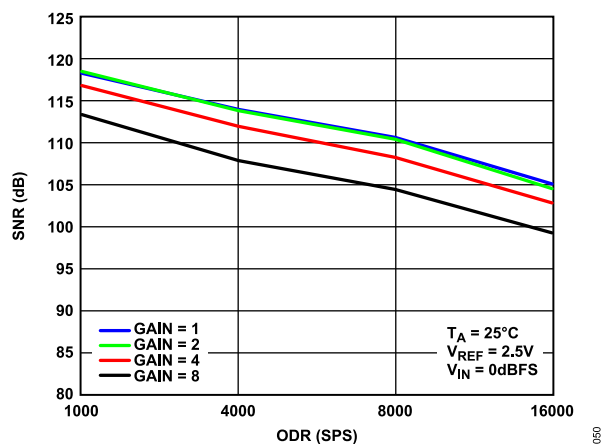
Figure 50. SNR vs. ODR at 16 kSPS, High Resolution Mode ( AVDDx = 3.6\text{ V} , IOVDD = 3.6\text{ V} )
