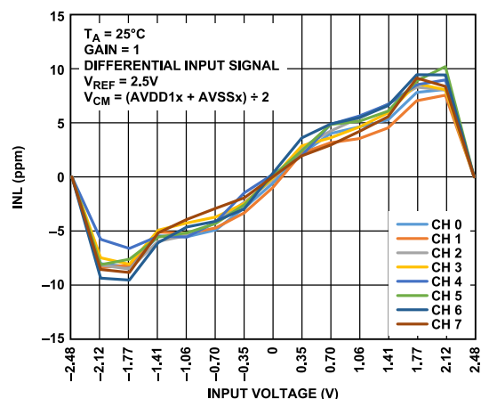
Figure 11. INL vs. Input Voltage and Channel at 16 kSPS, Low Power Mode
