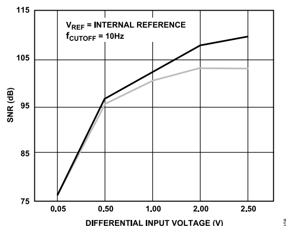
Figure 108. SNR Adding External LPF with V_{\text{REF}} = \text{Internal Reference} and f_{\text{CUTOFF}} = 10 Hz
