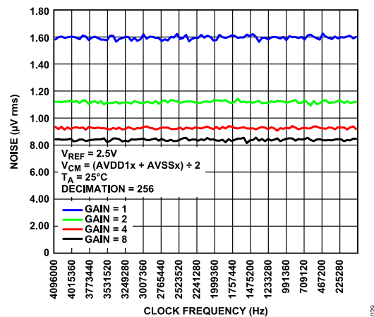
Figure 29. Noise vs. Clock Frequency, Low Power Mode
