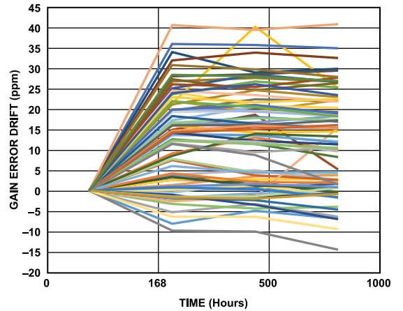
Figure 65. Gain Error Drift vs. Time
