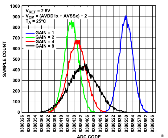
Figure 16. Noise Histogram at 16 kSPS, High Resolution Mode, Sinc3 Filter Enabled
