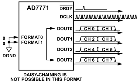
Figure 131. FORMATx Pin Configuration—FORMAT0 = 0, FORMAT1 = 0
