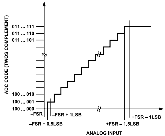
Figure 106. Transfer Function
