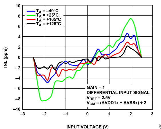
Figure 10. INL vs. Input Voltage and Temperature at 64 kSPS, High Resolution Mode
