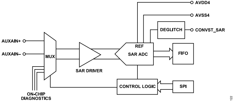
Figure 123. SAR ADC Configuration and Control
