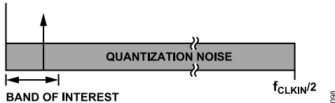
Figure 98. \Sigma - \Delta ADC Operation, Reduction of Noise Energy Contained in the Band of Interest (Linear Scale X-Axis)
