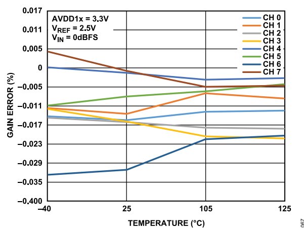
Figure 67. Gain Error vs. Temperature, Low Power Mode
