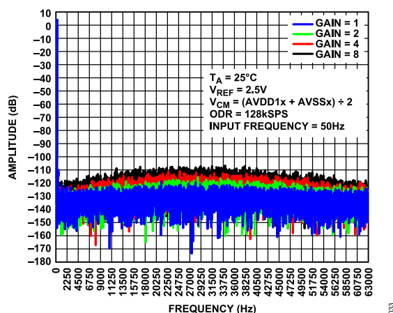
Figure 33. FFT Plot, High Resolution Mode at 128 kSPS, Input Frequency ( f_{IN} ) = 50 Hz, Sinc5 Filter Enabled
