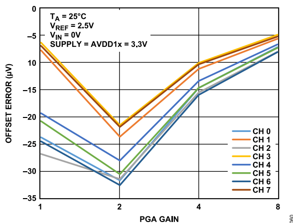
Figure 60. Offset Error vs. PGA Gain at 16 kSPS, Low Power Mode
