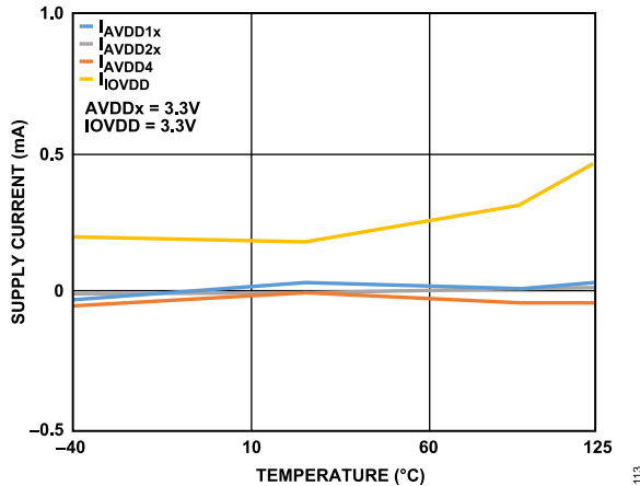
Figure 113. Shutdown Current
