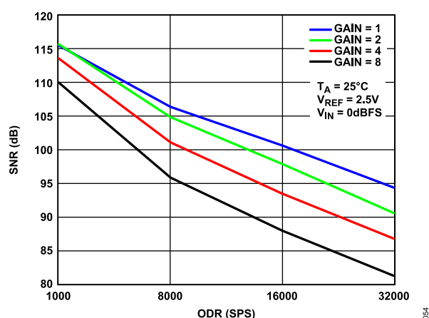
Figure 54. SNR vs. ODR at 16 kSPS, Low Power Mode ( AVDDx = 3.6\text{ V} , IOVDD = 3.6\text{ V} )
