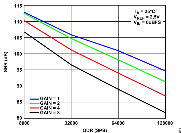
Figure 51. SNR vs. ODR at 64 kSPS, High Resolution Mode ( AVDDx = 3.6\text{ V} , IOVDD = 3.6\text{ V} )
