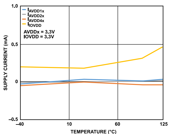
Figure 97. Shutdown Current
