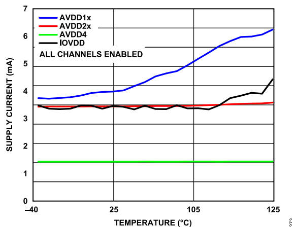
Figure 73. Supply Current vs. Temperature, Low Power Mode
