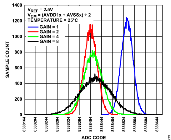
Figure 19. Noise Histogram at 4 kSPS, Low Power Mode
