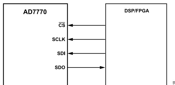
Figure 101. SPI Control Interface—AD7770 is the SPI Subordinate, Digital Signal Processor (DSP)/Field Programmable Gate Array (FPGA) is the Main
