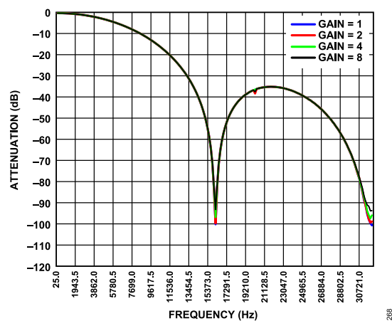
Figure 68. Filter Profiles at 16 kSPS, High Resolution Mode
