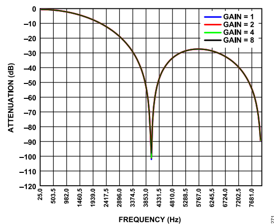
Figure 71. Filter Profiles at 4 kSPS, Low Power Mode
