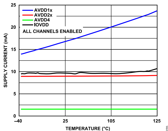
Figure 70. Supply Current vs. Temperature, High Resolution Mode
