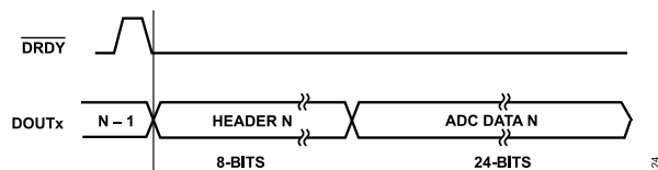
Figure 108. ADC Output—8-Bit Header Plus 24-Bit Conversion Data
