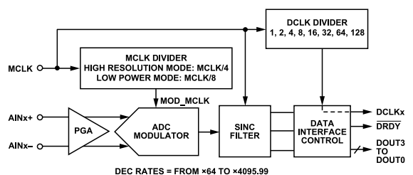
Figure 94. Clock Generation on the AD7770
