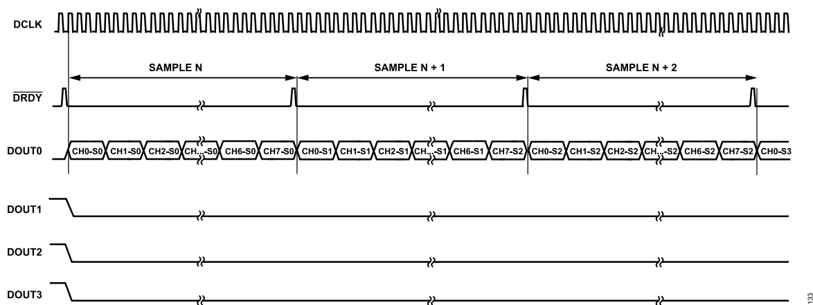
Figure 118. FORMAT0 = 1 , FORMAT1 = 0 —Channel 0 to Channel 7 Output on DOUT0 Only (S0 Means Sample 0 and S1 Means Sample 1)
