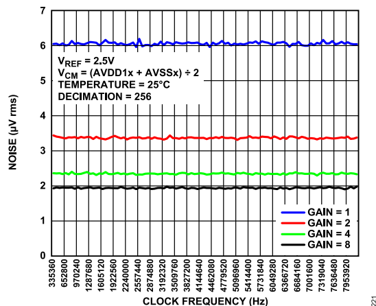
Figure 21. Noise vs. Clock Frequency, High Resolution Mode
