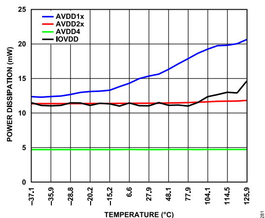
Figure 81. Power Dissipation vs. Temperature, Low Power Mode
