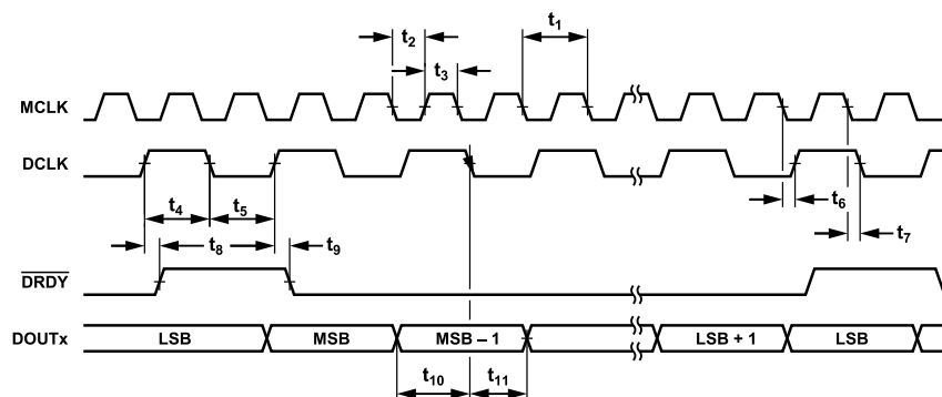
Figure 2. Data Interface Timing Diagram
