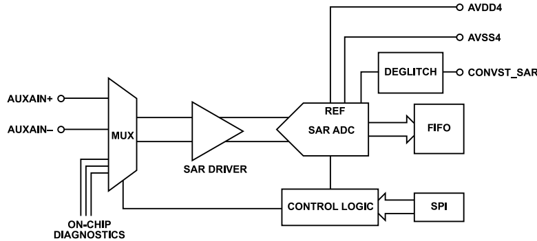
Figure 107. SAR ADC Configuration and Control
