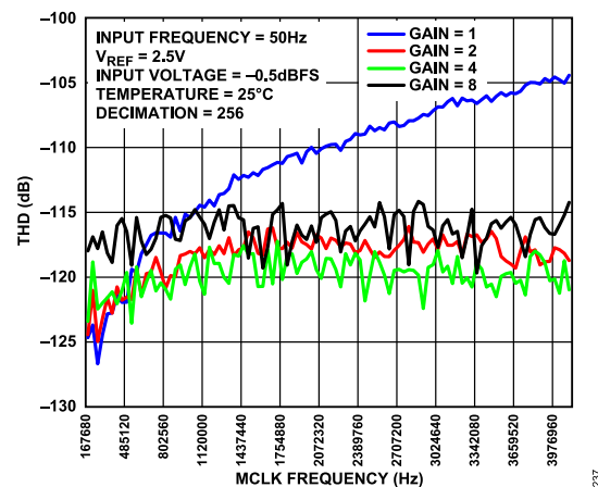
Figure 37. THD vs. MCLK Frequency, Low Power Mode
