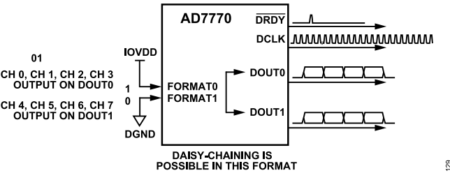
Figure 114. FORMATx Pin Configuration—FORMAT0 = 1, FORMAT1 = 0
