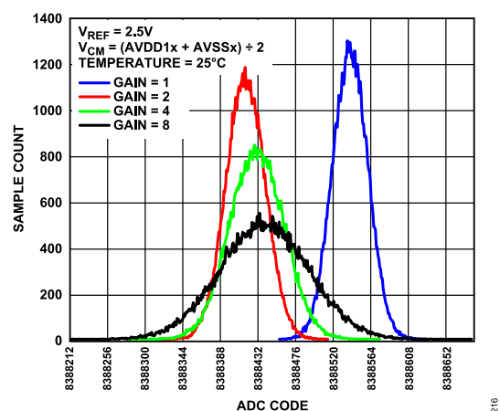
Figure 16. Noise Histogram at 16 kSPS, High Resolution Mode
