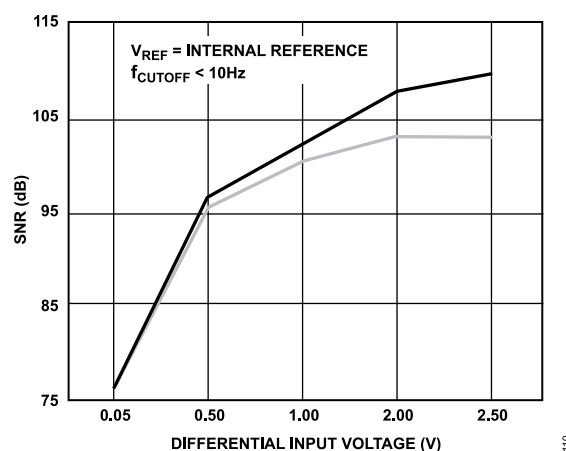
Figure 93. SNR Adding External LPF with V_{\text{REF}} = \text{Internal Reference} and f_{\text{CUTOFF}} < 10 Hz
