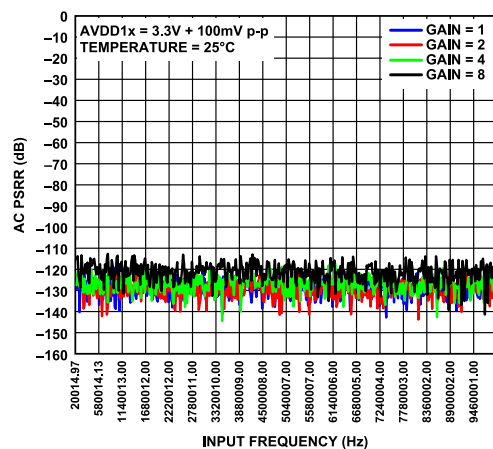
Figure 67. AC PSRR vs. Input Frequency at 4 kSPS, Low Power Mode
