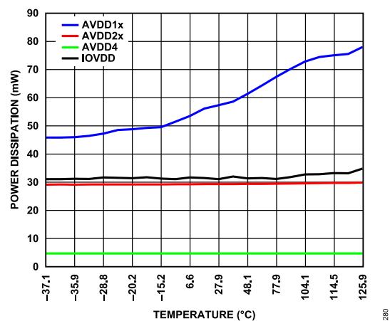
Figure 80. Power Dissipation vs. Temperature, High Resolution Mode
