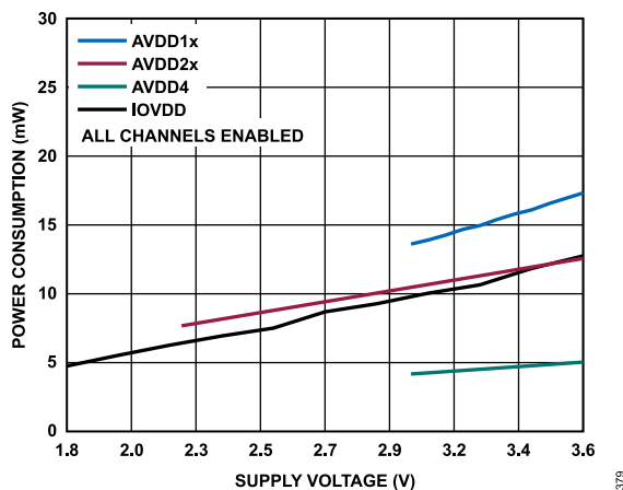
Figure 79. Power Consumption vs. Supply Voltage, Low Power Mode
