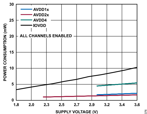
Figure 76. Power Consumption vs. Supply Voltage, High Resolution Mode
