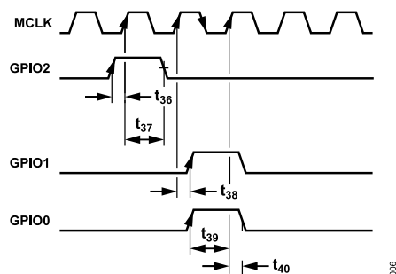
Figure 6. GPIOs for SRC Update Timing Diagram
