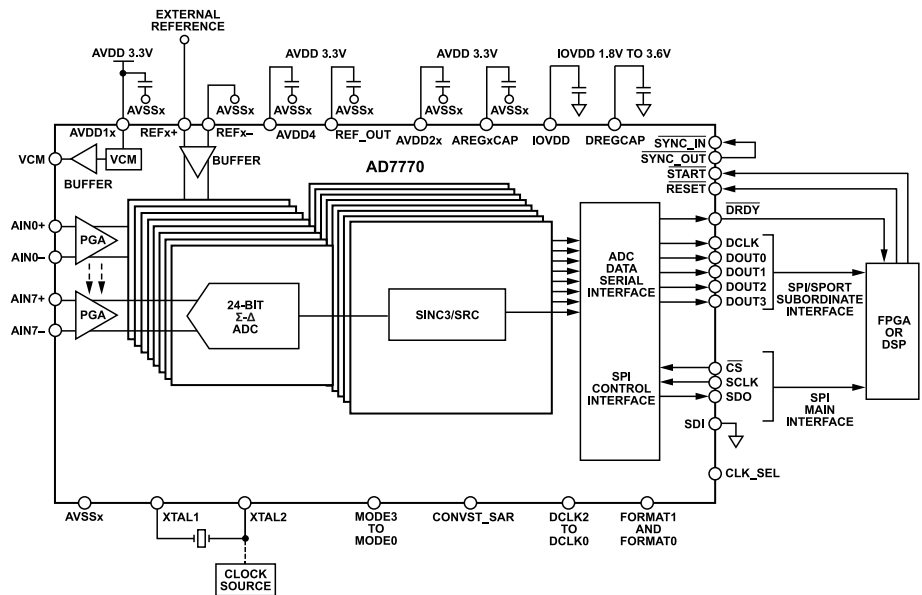
Figure 98. Pin Mode Connection Diagram with External Reference
