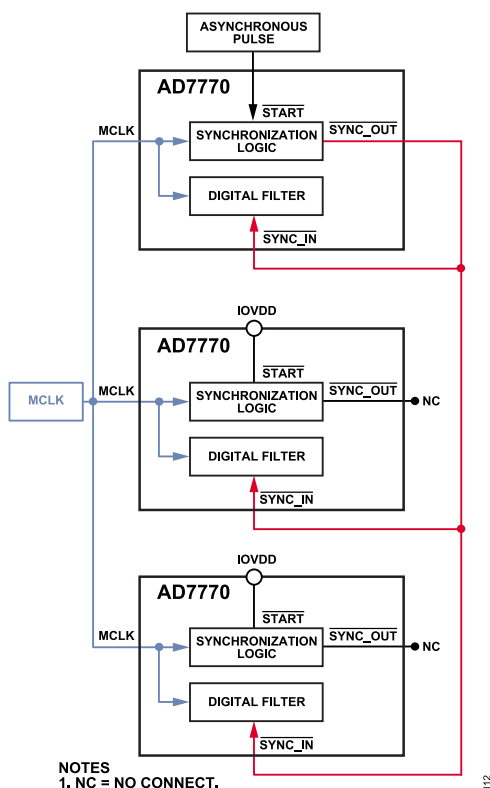
Figure 95. Multiple AD7770 Devices Synchronization
