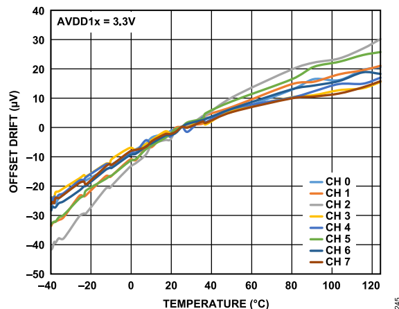
Figure 45. Offset Drift vs. Temperature
