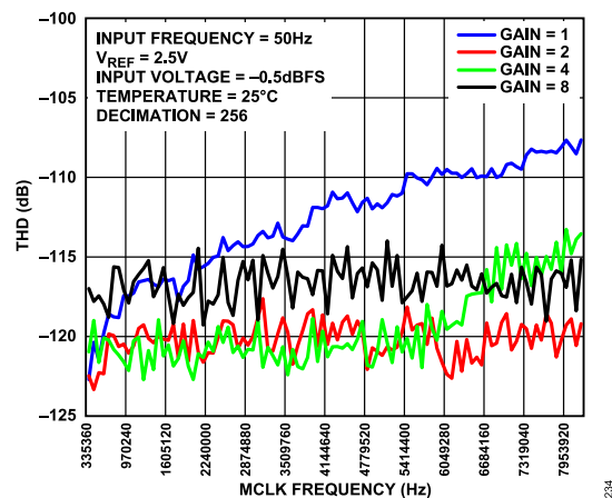
Figure 34. THD vs. MCLK Frequency, High Resolution Mode
