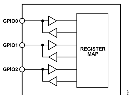
Figure 100. GPIOx Pin Functionality
